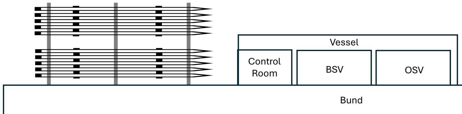
Front View
